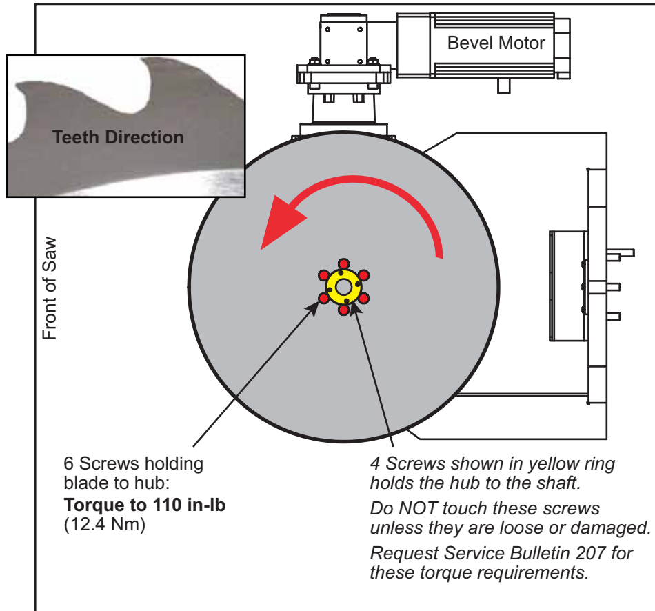
Figure 3: Torque Specs for Saw Blade (View from side of saw, with blade at 90 degrees.)
